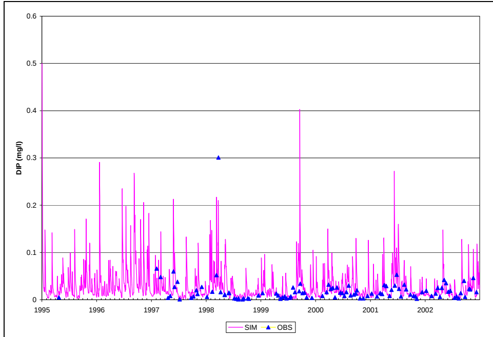
Figure B.41. Time Series of Observed and Simulated DIP, Calibration Scenario, ANA14
