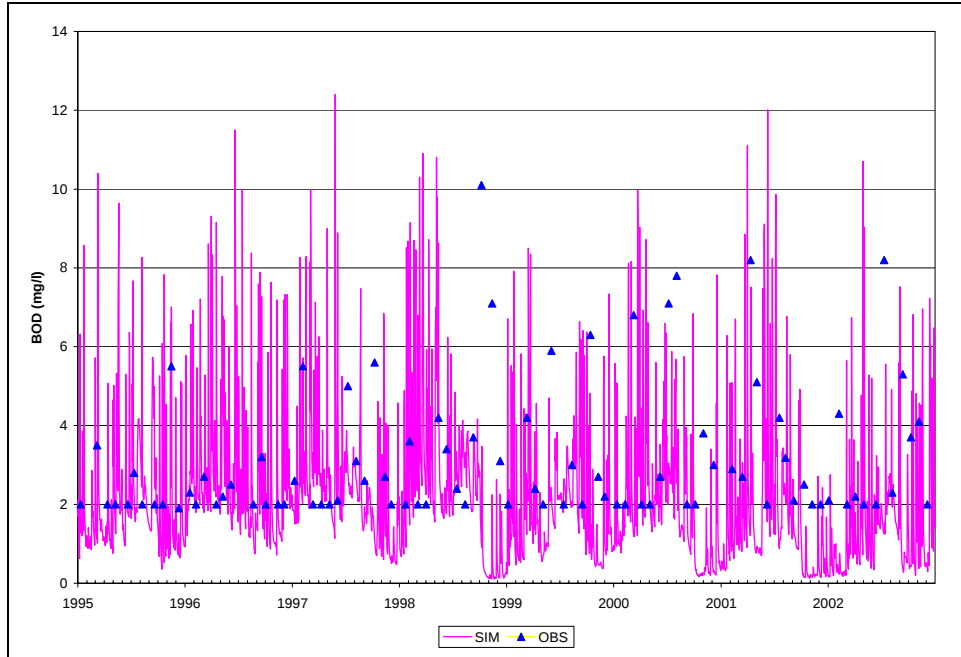
Figure B.19. Time Series of Observed and Simulated BOD5, Calibration Scenario, ANA0082
