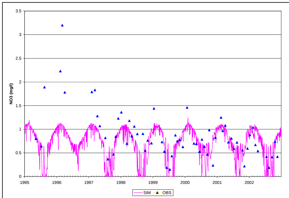
Figure B.32. Time Series of Observed and Simulated NO3-N, Calibration Scenario, ANA30
