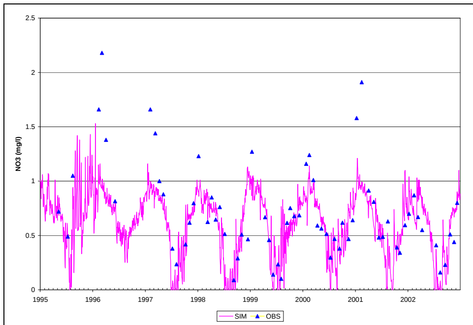
Figure B.34. Time Series of Observed and Simulated NO3-N, Calibration Scenario, ANA08
