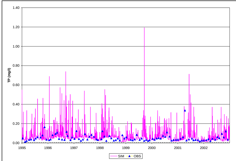
Figure B.37. Time Series of Observed and Simulated TP, Calibration Scenario, ANA0082
