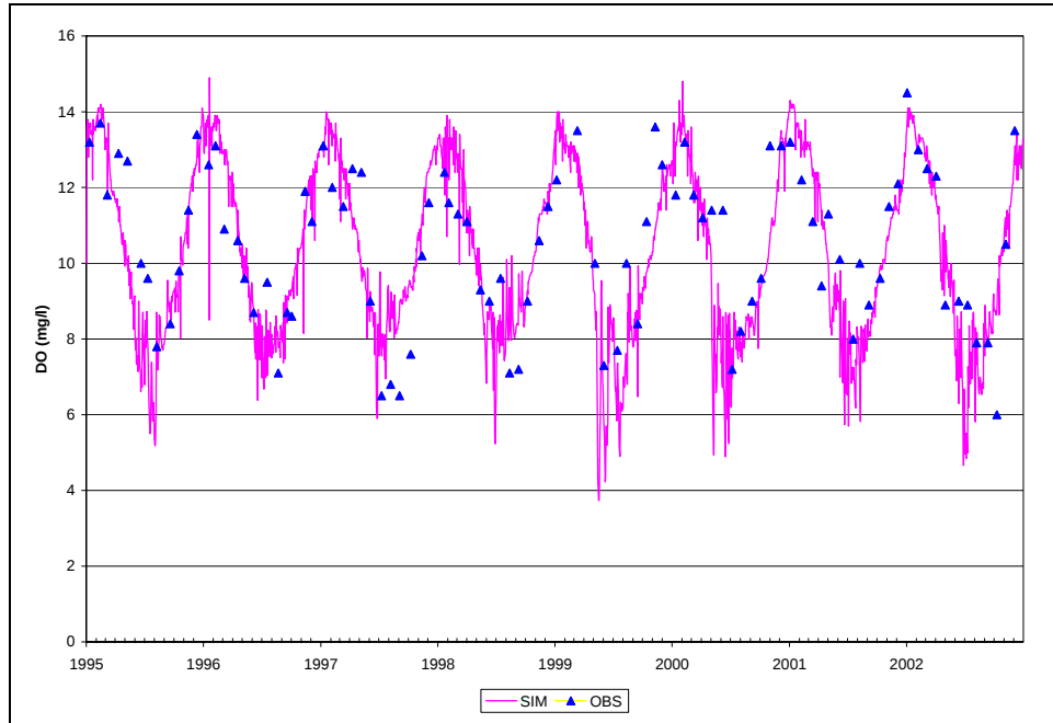
Figure B.1. Time Series of Observed and Simulated DO, Calibration Scenario, ANA0082
