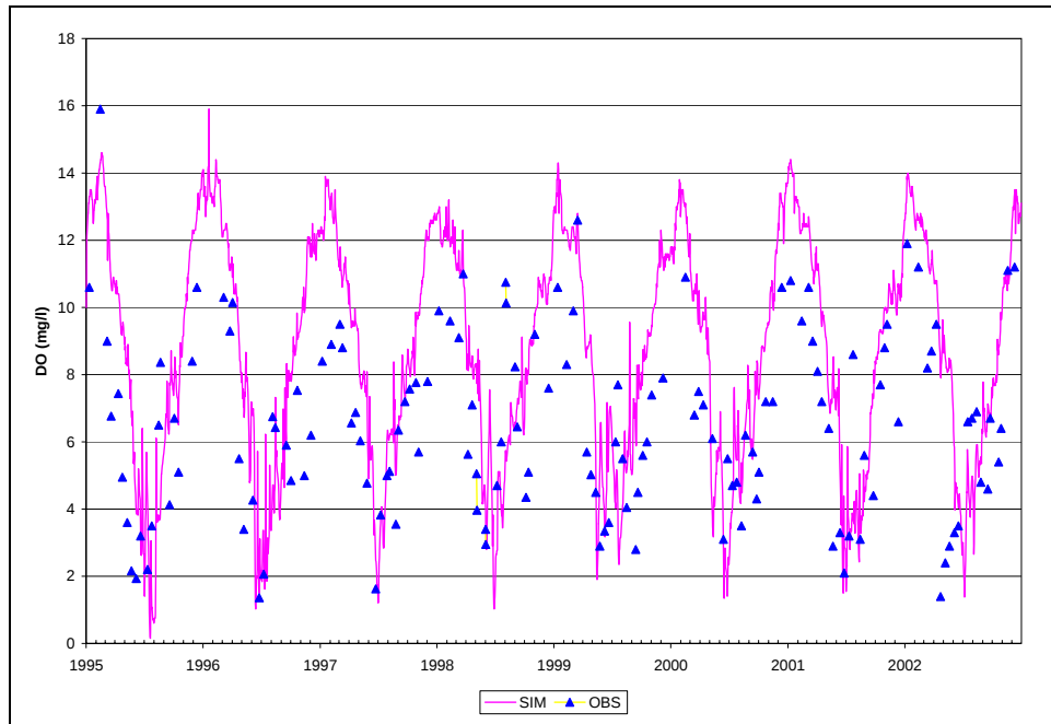
Figure B.5. Time Series of Observed and Simulated DO, Calibration Scenario, ANA14
