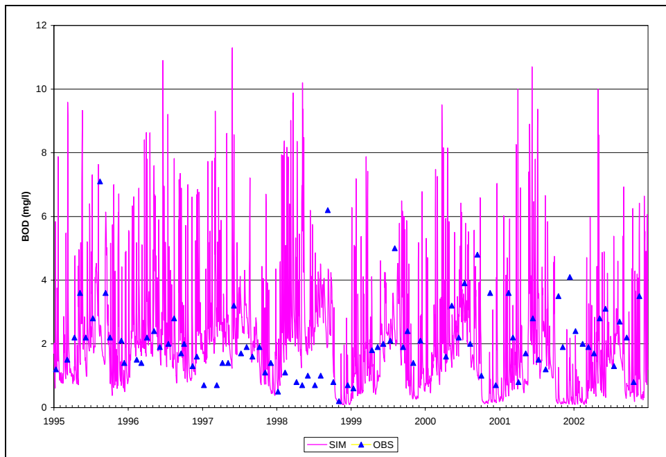
Figure B.20. Time Series of Observed and Simulated BOD5, Calibration Scenario, ANA30
