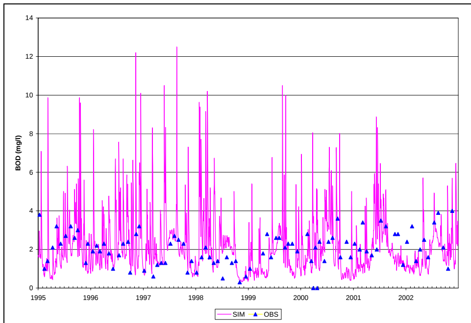
Figure B.24. Time Series of Observed and Simulated BOD5, Calibration Scenario, ANA21
