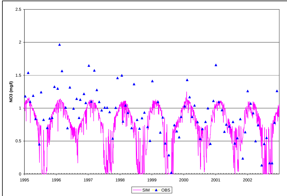
Figure B.31. Time Series of Observed and Simulated NO3-N, Calibration Scenario, ANA0082
