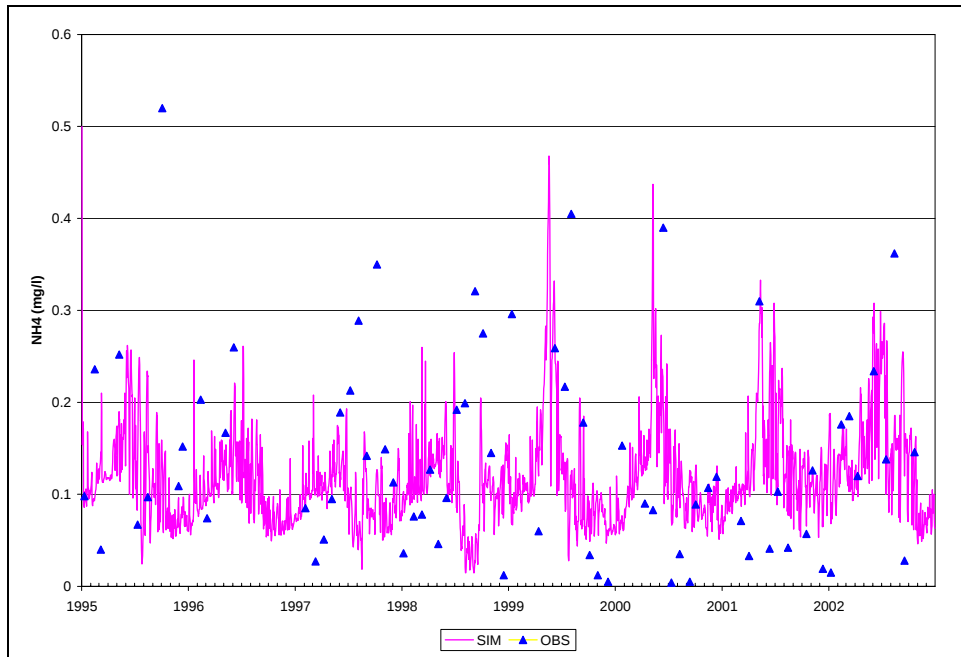
Figure B.26. Time Series of Observed and Simulated NH4-N, Calibration Scenario, ANA30
