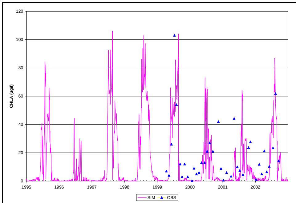
Figure B.10. Time Series of Observed and Simulated CHLA, Calibration Scenario, ANA08
