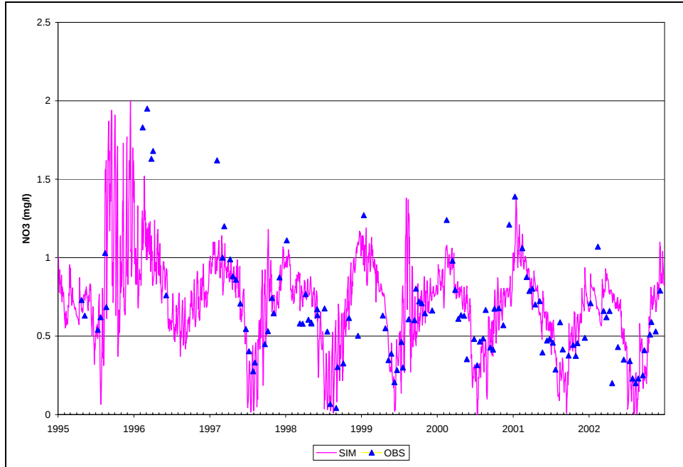
Figure B.35. Time Series of Observed and Simulated NO3-N, Calibration Scenario, ANA14
