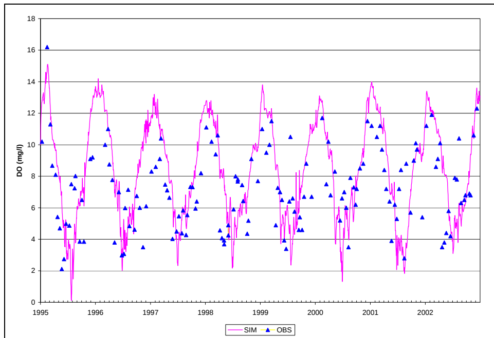
Figure B.6. Time Series of Observed and Simulated DO, Calibration Scenario, ANA21
