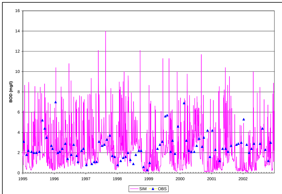
Figure B.22. Time Series of Observed and Simulated BOD5, Calibration Scenario, ANA08
