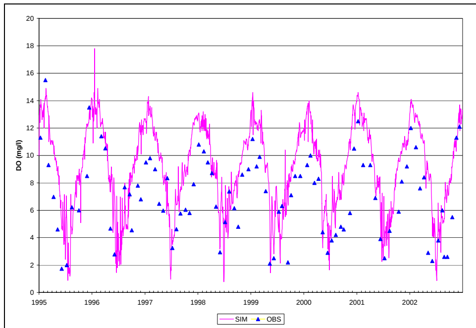
Figure B.4. Time Series of Observed and Simulated DO, Calibration Scenario, ANA08
