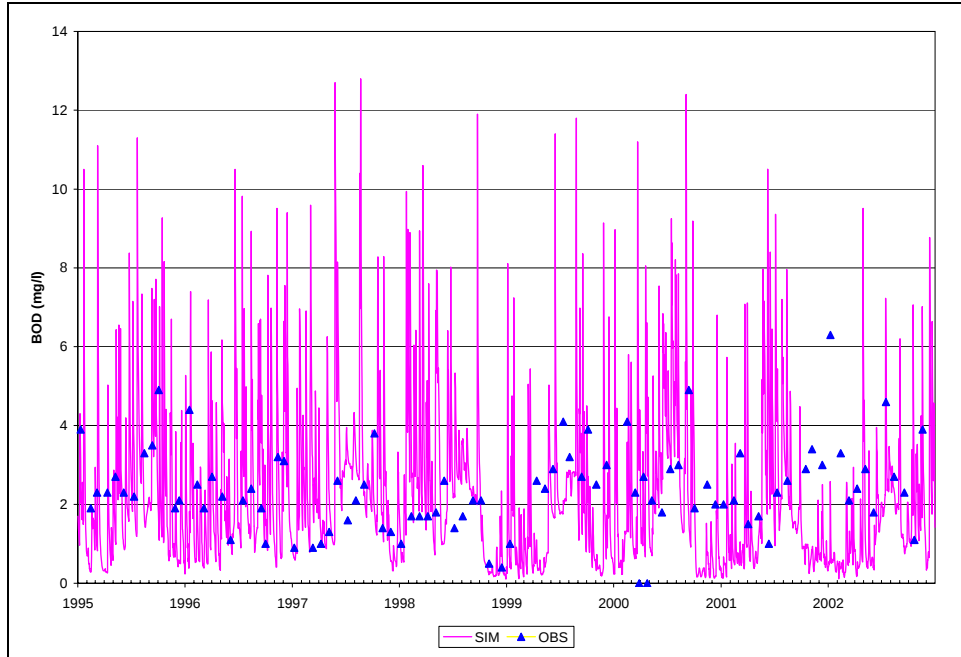
Figure B.23. Time Series of Observed and Simulated BOD5, Calibration Scenario, ANA14
