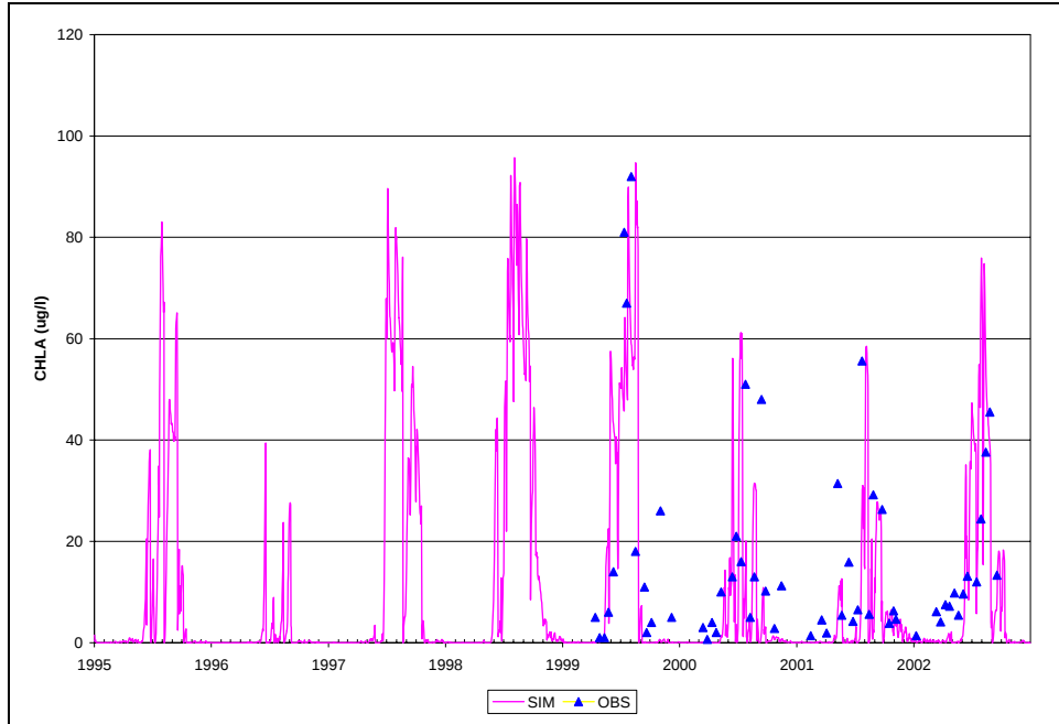
Figure B.9. Time Series of Observed and Simulated CHLA, Calibration Scenario, ANA01
