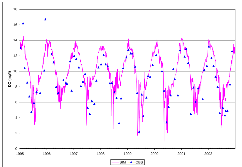
Figure B.2. Time Series of Observed and Simulated DO, Calibration Scenario, ANA30
