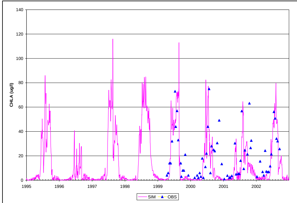
Figure B.11. Time Series of Observed and Simulated CHLA, Calibration Scenario, ANA14
