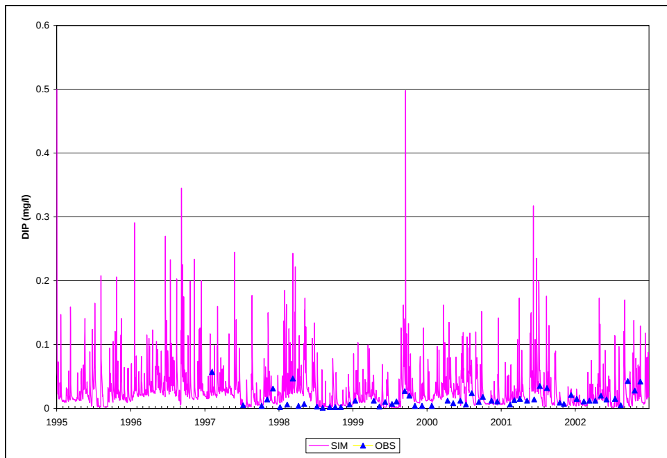
Figure B.38. Time Series of Observed and Simulated DIP, Calibration Scenario, ANA30
