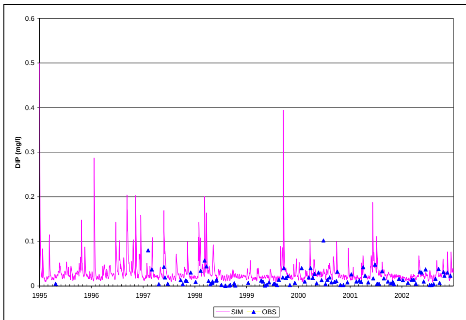
Figure B.42. Time Series of Observed and Simulated DIP, Calibration Scenario, ANA21
