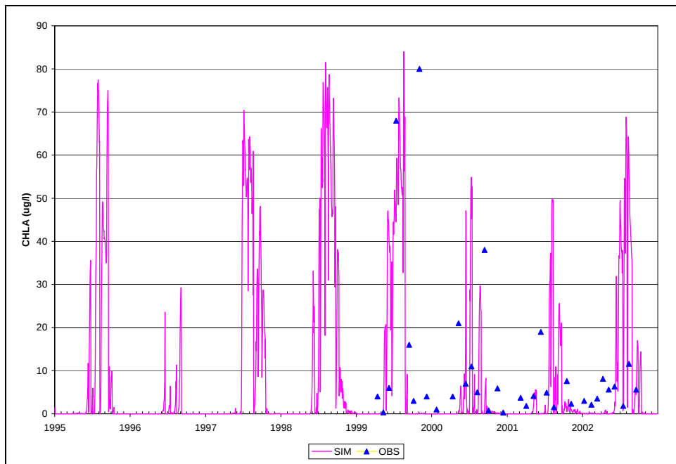
Figure B.8. Time Series of Observed and Simulated CHLA, Calibration Scenario, ANA30
