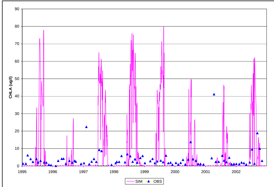
Figure B.7. Time Series of Observed and Simulated CHLA, Calibration Scenario, ANA0082
