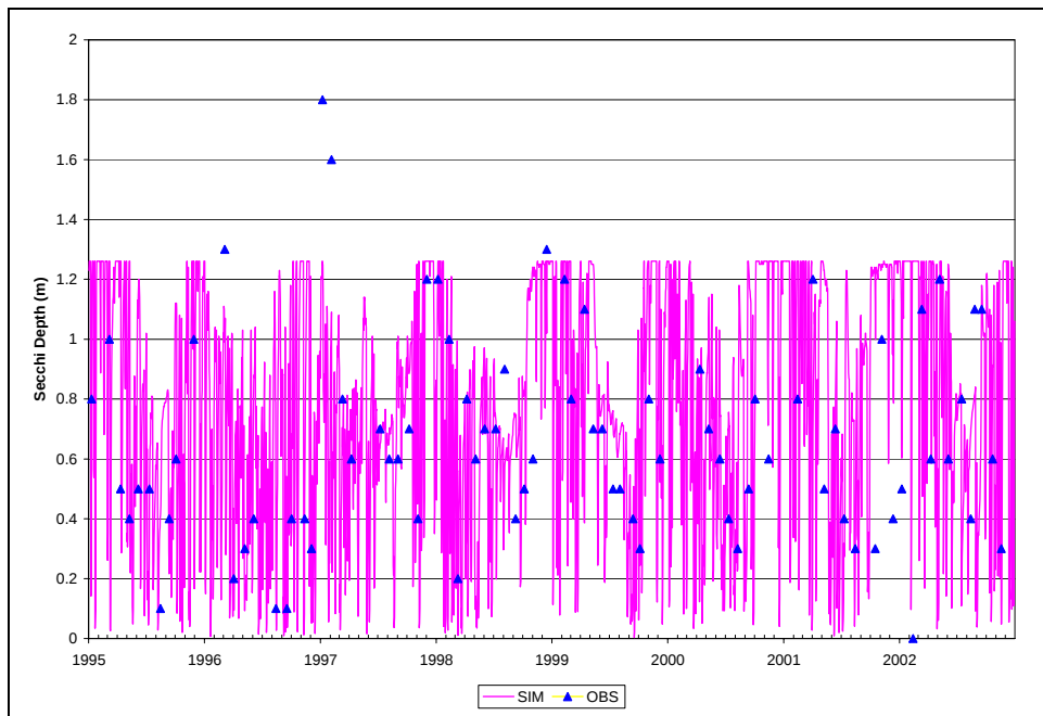
Figure B.14. Time Series of Observed and Simulated SECCHI DEPTH, Calibration Scenario, ANA30
