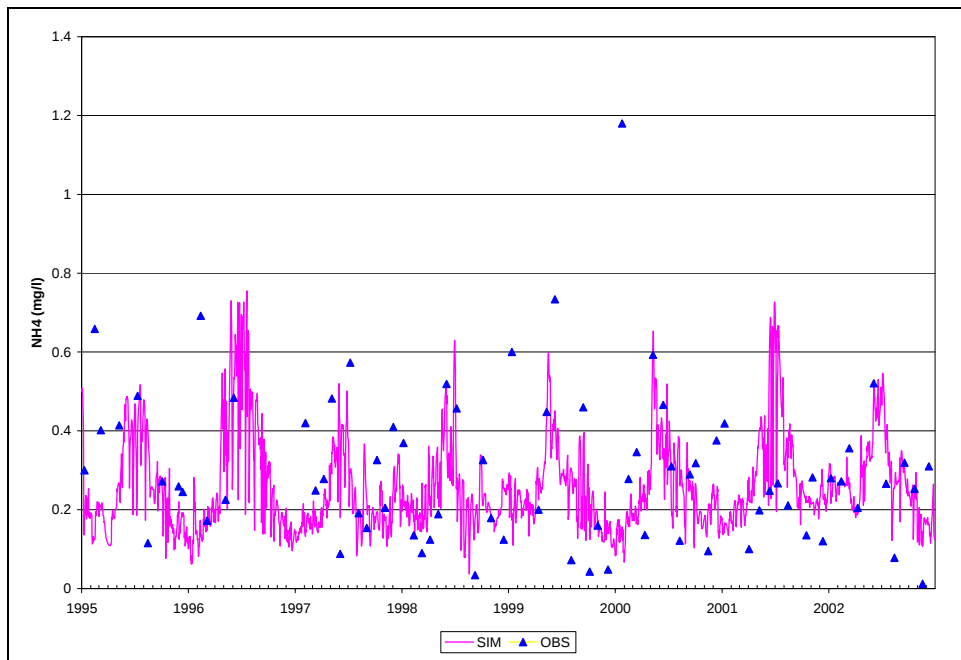
Figure B.28. Time Series of Observed and Simulated NH4-N, Calibration Scenario, ANA08
