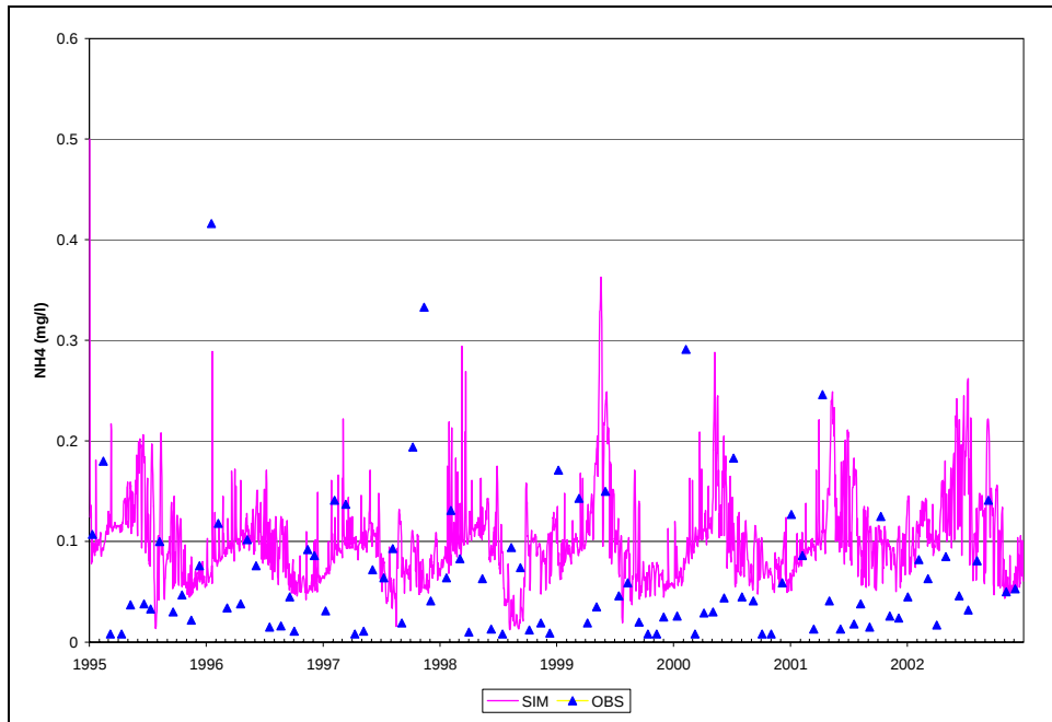
Figure B.25. Time Series of Observed and Simulated NH4-N, Calibration Scenario, ANA0082
