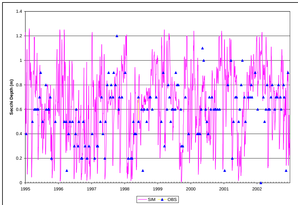
Figure B.18. Time Series of Observed and Simulated SECCHI DEPTH, Calibration Scenario, ANA21
