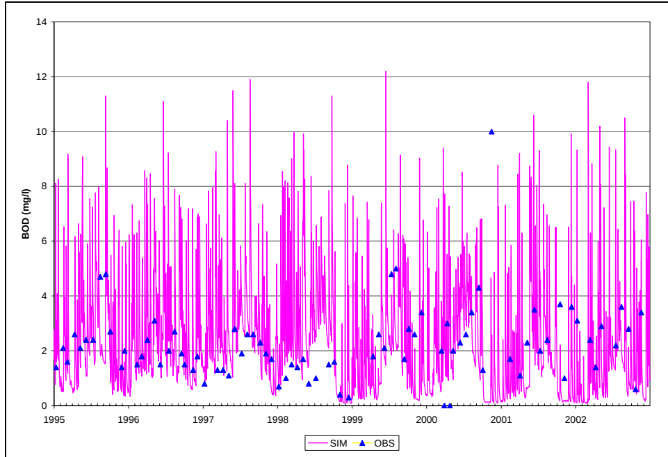
Figure B.21. Time Series of Observed and Simulated BOD5, Calibration Scenario, ANA01
