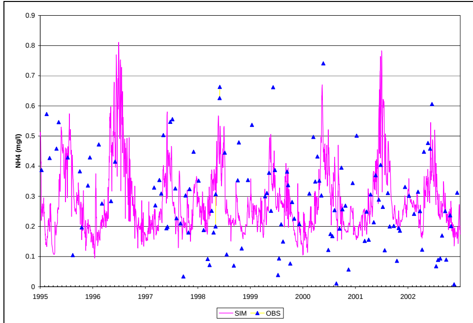
Figure B.29. Time Series of Observed and Simulated NH4-N, Calibration Scenario, ANA14
