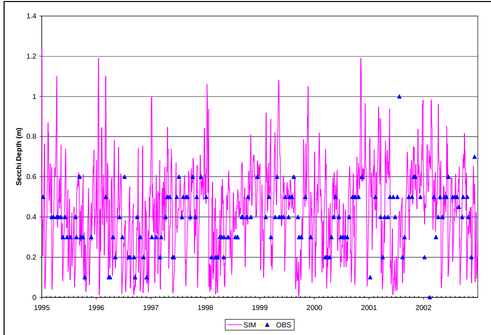
Figure B.17. Time Series of Observed and Simulated SECCHI DEPTH, Calibration Scenario, ANA14
