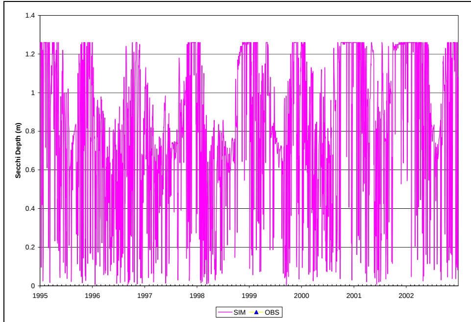
Figure B.13. Time Series of Simulated SECCHI DEPTH, Calibration Scenario, ANA0082
