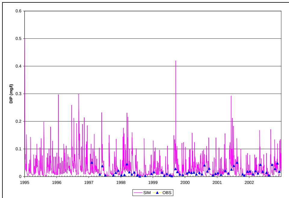
Figure B.40. Time Series of Observed and Simulated DIP, Calibration Scenario, ANA08
