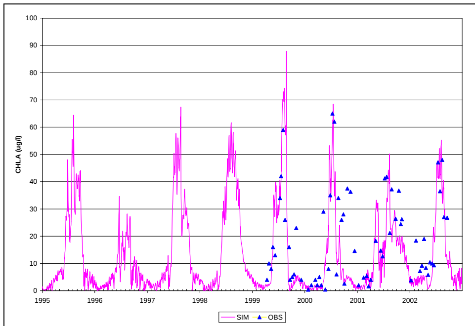
Figure B.12. Time Series of Observed and Simulated CHLA, Calibration Scenario, ANA21
