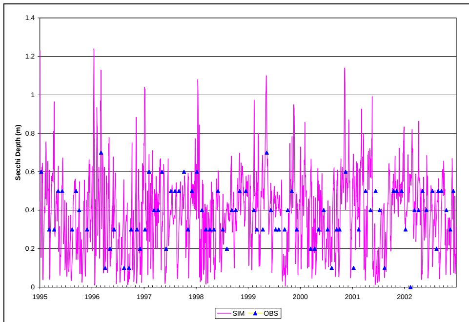
Figure B.16. Time Series of Observed and Simulated SECCHI DEPTH, Calibration Scenario, ANA08
