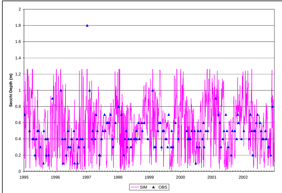
Figure B.15. Time Series of Observed and Simulated SECCHI DEPTH, Calibration Scenario, ANA01
