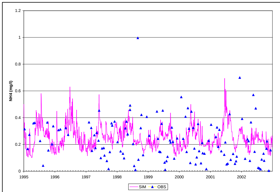
Figure B.30. Time Series of Observed and Simulated NH4-N, Calibration Scenario, ANA21
