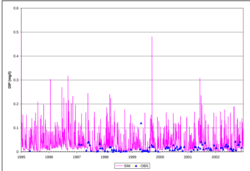
Figure B.39. Time Series of Observed and Simulated DIP, Calibration Scenario, ANA01
