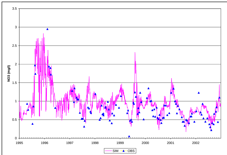
Figure B.36. Time Series of Observed and Simulated NO3-N, Calibration Scenario, ANA21
