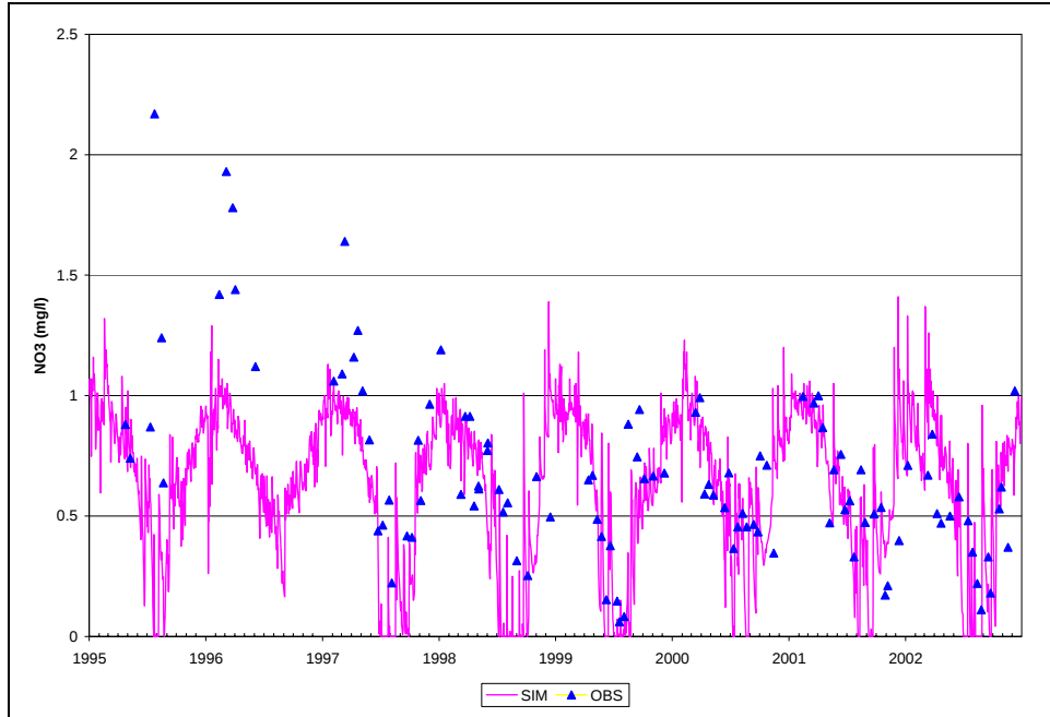
Figure B.33. Time Series of Observed and Simulated NO3-N, Calibration Scenario, ANA01
