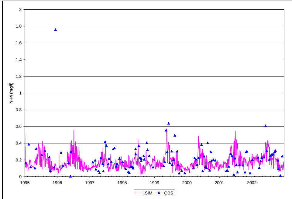
Figure B.27. Time Series of Observed and Simulated NH4-N, Calibration Scenario, ANA01
