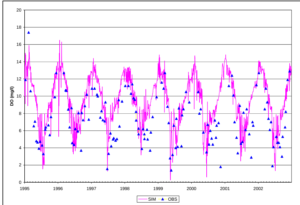
Figure B.3. Time Series of Observed and Simulated DO, Calibration Scenario, ANA01
